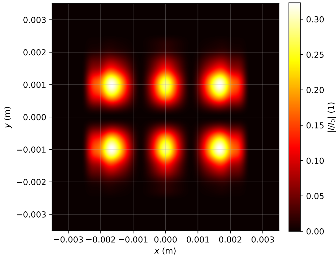
Intensity profile I(x, y, z = 3.742)/I_0 , P_{in}=2.0P_{cr} , artificial time
